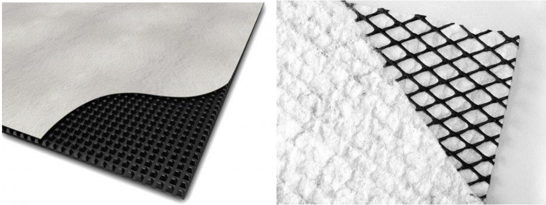
Image: Geocomposite Drain with a Cuspated Sheet (left) and Geonet (right)
