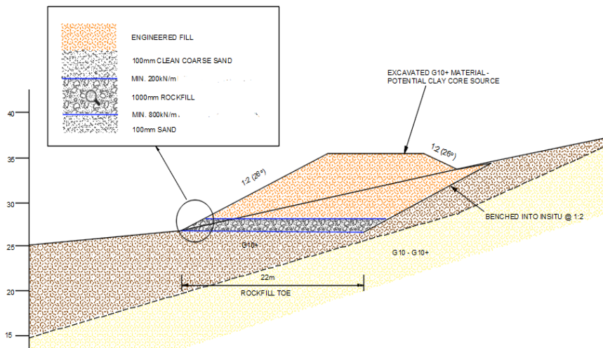
Figure 2: Cross section of Embankment at Zimbali Lakes
