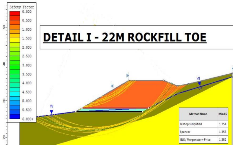
Figure 3: Cross section of Embankment with 22m rockfill toe
