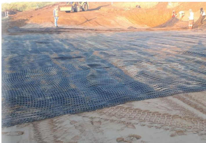
Figure 5: Tensioning of geogrid by hand
