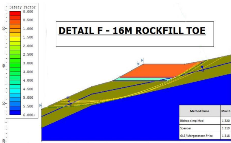
Figure 4: Cross section of Embankment with 16m rockfill toe
